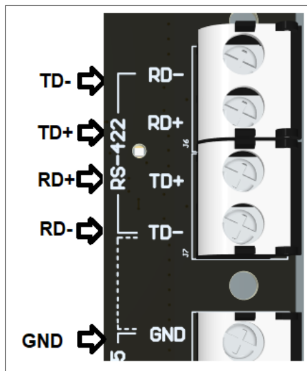
Figure 5. RS-422 connections
