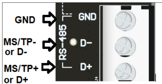
Figure 4. RS-485/BACnet connections
