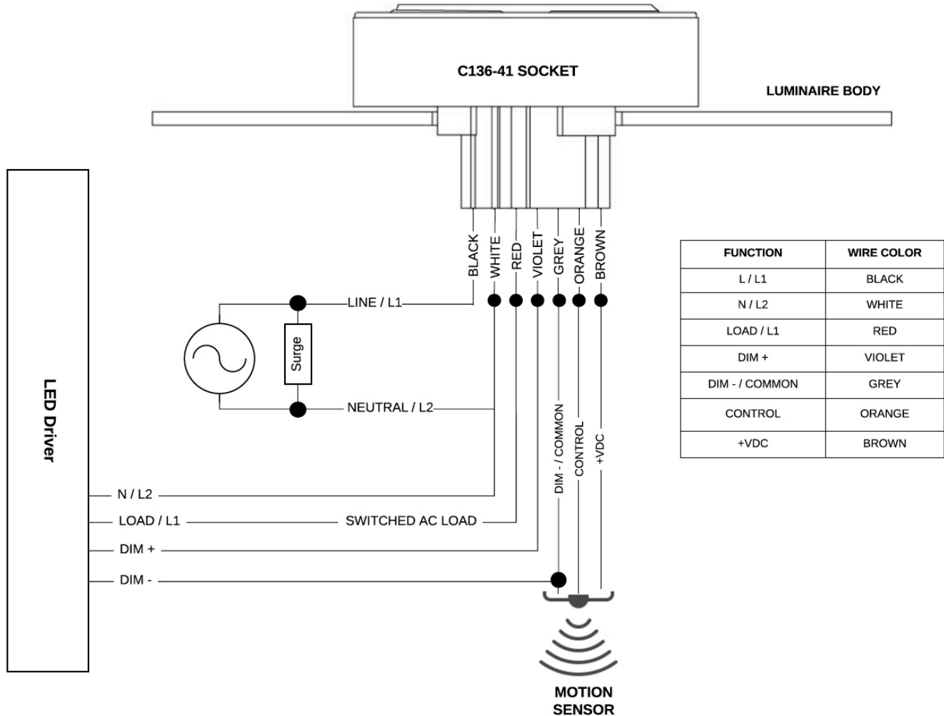
Figure 1 – C136-41 Socket Wiring Details
