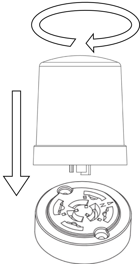
Figure 2 – Installation Diagram
